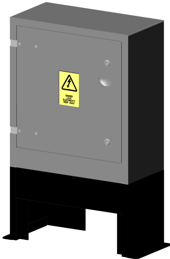
UP3-1P UNMETERED THREE/SINGLE PHASE PILLAR 600 WIDE HINGED DOOR
